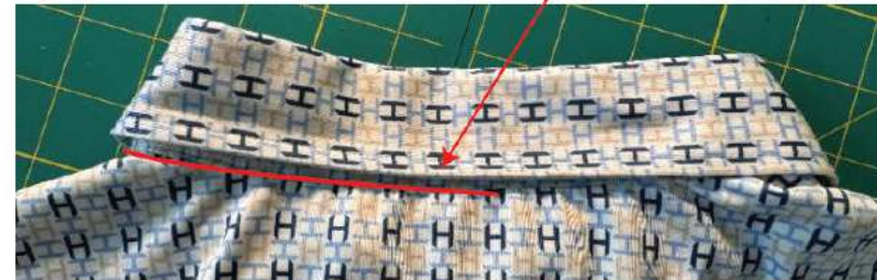
Collar roll is at band seam should be max of 1/4". Sample roll measures 1/2" and collar does not cover collar band seam in back.
